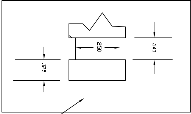
Groove Detail
